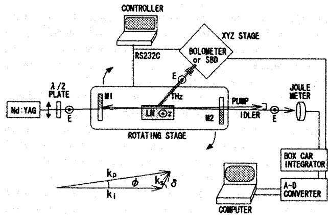
Fig. 20. Terahertz generator based on laser illumination of a lithium–niobate crystal (courtesy of [196], American Institute of Physics).
