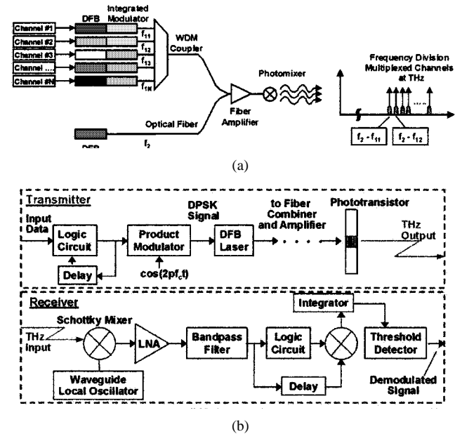
Fig. 10. (a) Optically diphexed terahertz transmitter source based on 1.5- \mu\text{m} fiber technology and terahertz power generation through photomixing. (b) Gigabit data-rate transmit/receive module based on this technology (courtesy of [52]).
