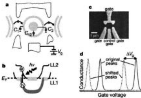
Fig. 17. Komiya quantum-dot single-photon detector concept (courtesy of [137]).
